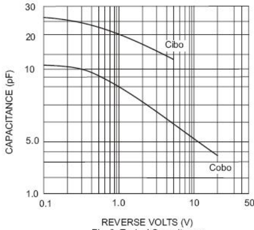
Fig. 3 Typical Capacitance
