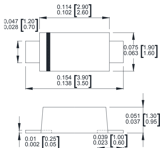
Dimensions : inch [ mm ]
