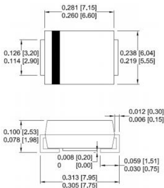
SMC/ DO-214AB
