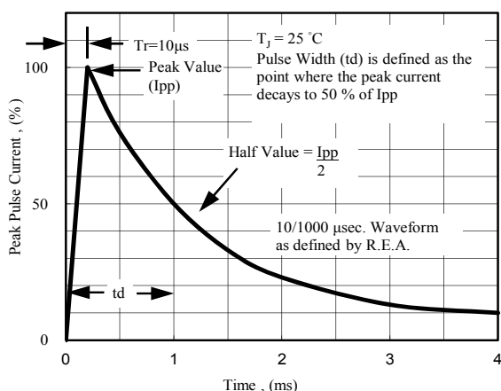
Fig. 5 - Pulse Waveform
