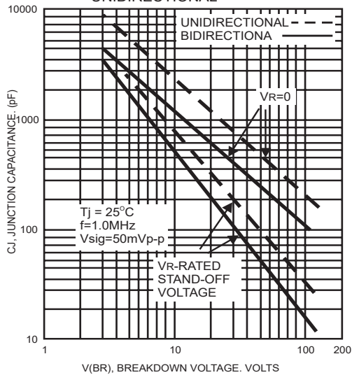
FIG.5- TYPICAL JUNCTION CAPACITANCE UNIDIRECTIONAL
